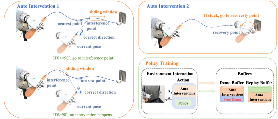
Fig. 1: Overview of AutoSERL. Auto Intervention 1 (Sliding Window Intervention): the robot is guided to the nearest point within the sliding window only when the angle \theta between the trajectory’s forward direction and the vector to that point satisfies \theta \leq 90^\circ , preventing the robot from being pulled back to already-visited positions. Auto Intervention 2 (Safety Recovery Mechanism): when the robot is stuck, it is guided to the recovery point and the demonstration segment is replayed to restore progress. Policy Training: intervention-guided transitions and the single human demonstration are stored in the Demo Buffer and Replay Buffer for policy training.
